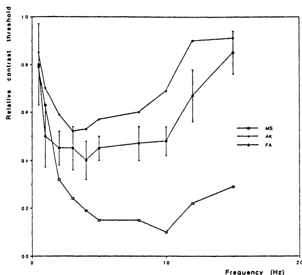
Figure 9: Flicker threshold.
