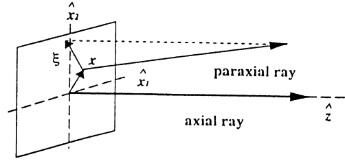
Figure 5: Ray coordinate.
