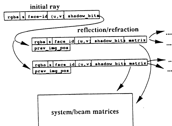
Figure 7: Data structure.
