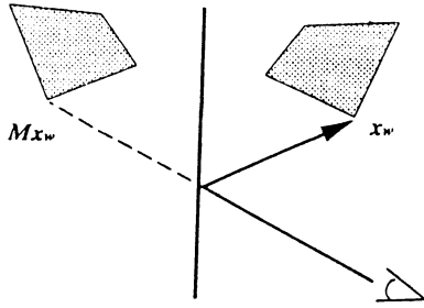
Figure 4: Beam tracing.
